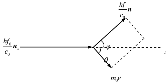
Figure 1 Model analysis of Compton effect
