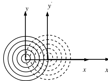
Fig.3 Light Source in Static System
