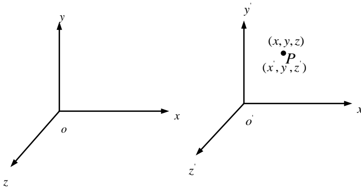
Fig. 1 Two Axis Frames with Relative Speed V
