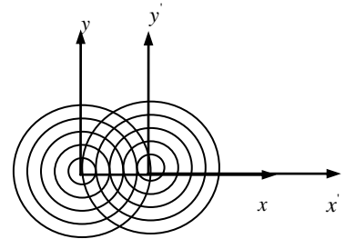
Fig.4 Two axis frames flash Simultaneously
