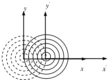
Fig.2 Light Source in Dynamic System
