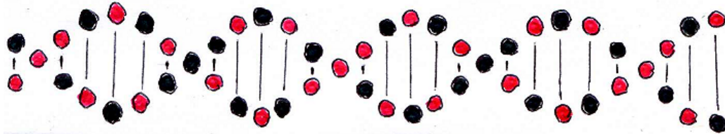
Fig. 1 A close-up view of a single magnetic line of force. The electrons are shown in red and the positrons are shown in black. The double helix is rotating about its axis with a prodigious angular speed, and the rotation axis represents the magnetic field vector H . The diagram is not drawn to scale since the relative dimensions remain unknown.
