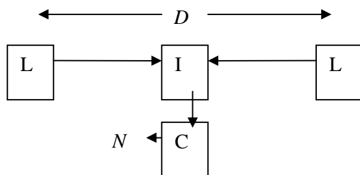
Fig 7 Detecting Sagnac effect on a rotating platform L=Laser C=Counter I=Interferometer N=Output from counter (or phase-detector)
