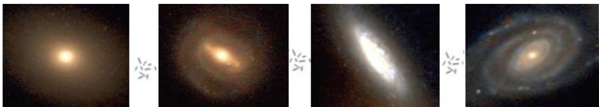
Fig.1.1 : The evolution of a spherical galaxy towards a spiral galaxy.
