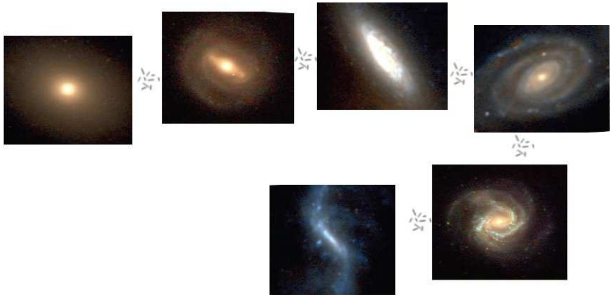
Fig.4.1: Evolutionary classification of galaxies. From spherical galaxy to an elliptic galaxy, then a disc galaxy and a spiral galaxy. After a reorientation of the bulge's angular momentum, a bar galaxy with a circularly outside-spreading turbulent zone is created, which a apocalyptic disturbance of the stars and planetary systems of the whole galaxy.
