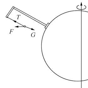
Fig 5.1 The sketch map of Eötvös experiment
