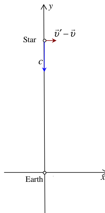
Fig 1.4 Observing star in the Earth's reference frame
