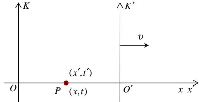
Fig 4.2 An simple event
