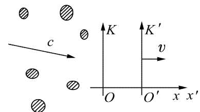
Fig 1.1 Is the light dependent on the frame of reference?
