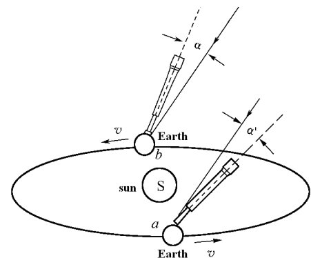
Fig 1.3 light aberration phenomenon
