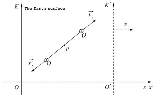
Fig 2.2 The observation of double charges in the frame K
