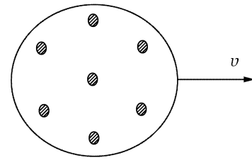
Fig 5.3 The sketch map of the particle structure
