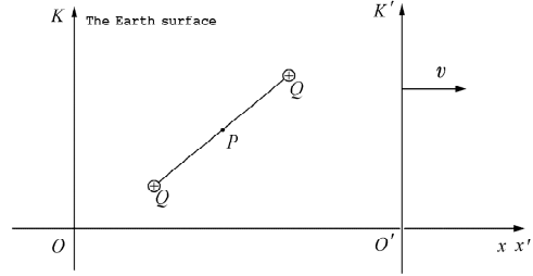
Fig 2.1 The systems of double charges and the two frames of reference
