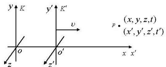
Fig 3.1 The sketch map of Lorentz Transformation
