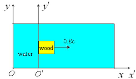
Fig 5.2 The sketch map of floating wood block
