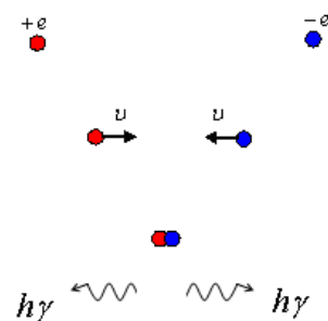
Fig 5.4 The sketch map of annihilation of electron and positron
