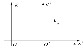
Fig 1.2 Where to study the velocity negating classical physics?
