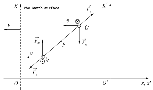
Fig 2.3 The observation of double charges in the frame K'
