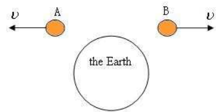
Fig 3.2 The sketch map of Twins Paradox
